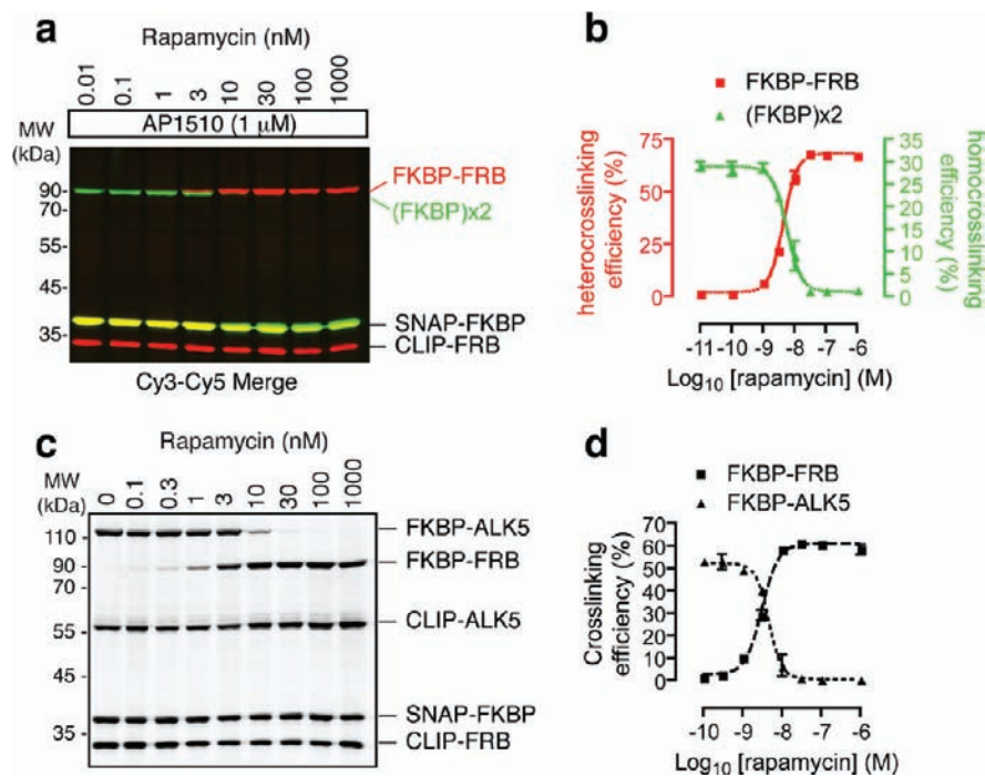
Figure 4. Simultaneous detection of several protein–protein interactions. (a,b) HEK 293 cells coexpressing SNAP-FKBP and CLIP-FRB were treated for 1 h with 1 μM AP1510 and different concentrations of rapamycin prior to lysis in the presence of 2 μM SC-Cy5 and 1 μM SS-Cy3. (a) Analysis of cross-linking by SDS-PAGE and in-gel fluorescence scanning; overlay of Cy3 (green) and Cy5 (red) channels. (b) Cross-linking efficiencies (mean ± SD of three independent experiments) determined in (a) versus rapamycin concentration. (c,d) HEK 293 cells coexpressing SNAP-FKBP, CLIP-FRB, and CLIP-ALK5 were treated for 1 h with different concentrations of rapamycin prior to lysis in the presence of 4 μM SC-Cy5. (c) Analysis of cross-linking by SDS-PAGE and in-gel fluorescence scanning. (d) Cross-linking efficiency (mean ± SD of two independent experiments) determined in (c) versus rapamycin concentration. (b and d) Data were fitted with sigmoidal dose–response equations.
